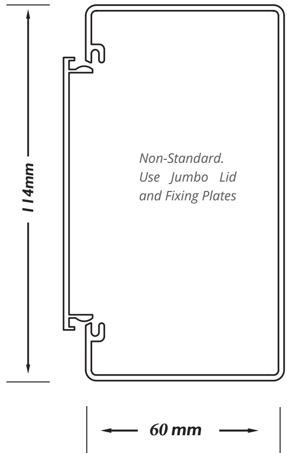
PDL 591CP Conversion Unit to allow standard power and data fittings (supply by others).
