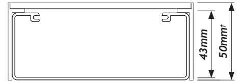
CAT 5 115.18.50 MINIMUM DEPTH & CONFIGURATION
