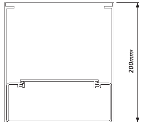
CAT 5 115.18.200 MAXIMUM DEPTH & CONFIGURATION
