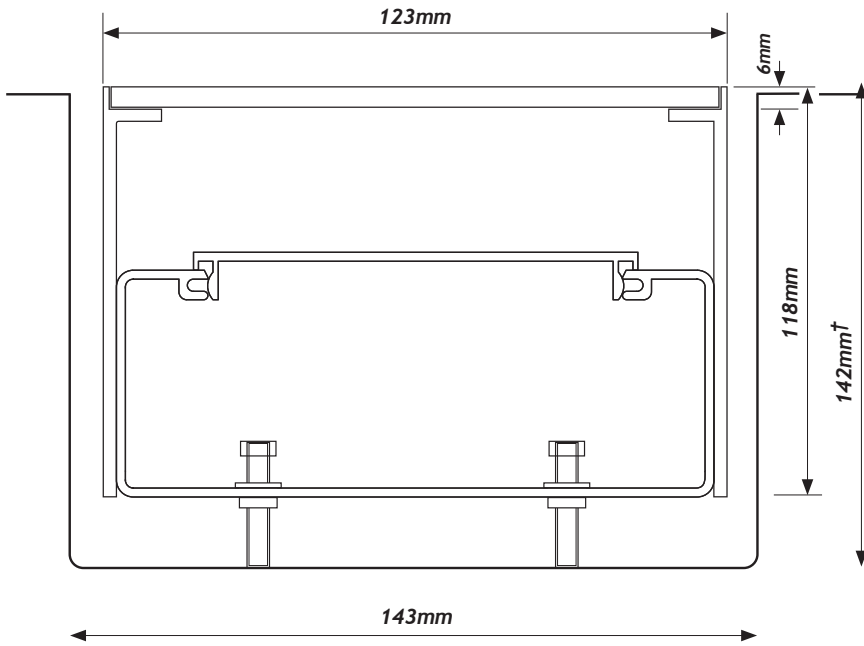
Double Compartment Floor Channel - CAT5/115/1 shown
