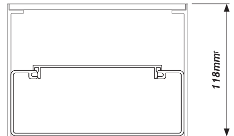
CAT 5 115.18.118 STANDARD DEPTH & CONFIGURATION
