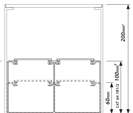
180x200.28 MAXIMUM DEPTH & CONFIGURATION
