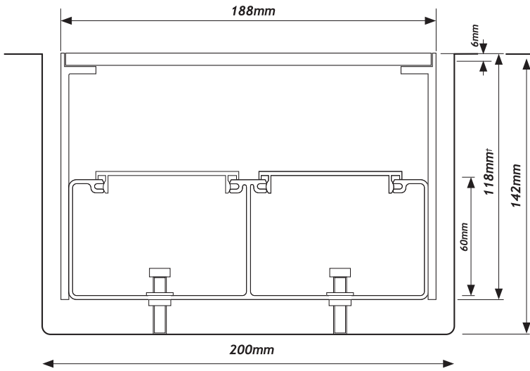
Double Compartment Floor Channel - 180x118/2 shown
